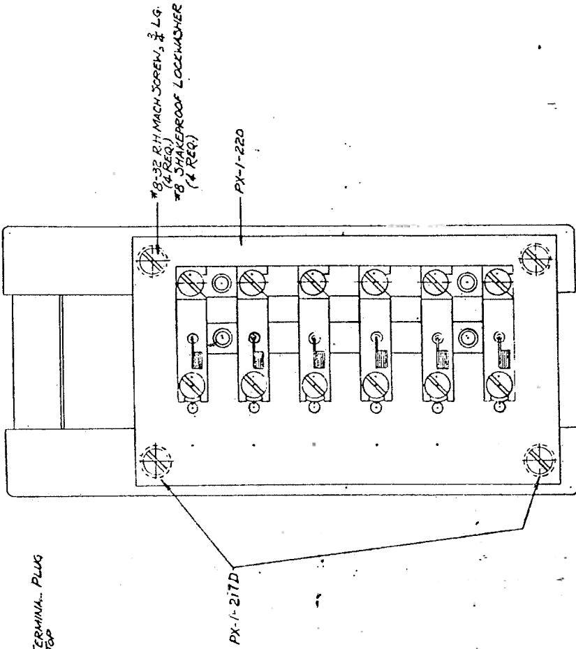
FUSE BLOCK MOUNTED ON TRANSFORMER COVER REMOVED
