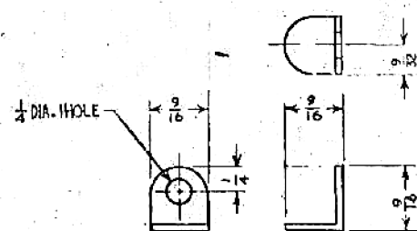
DETAIL OF GROUND LUG Scale - Full Size
