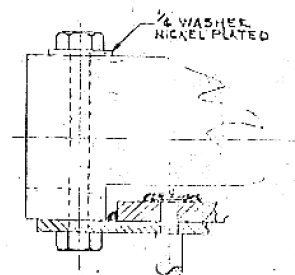
SECTION C-C (REF. SECT B-B) SCALE: FULL SIZE
