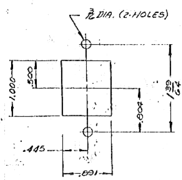
DETAIL N°1 FULL SIZE
