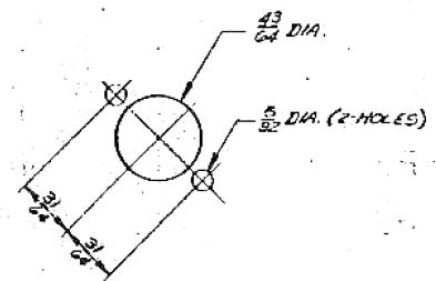
DETAIL N° 1 FULL SIZE
