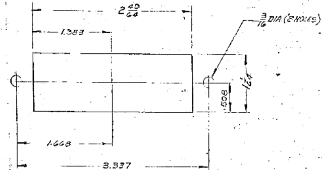
DETAIL N° 3 FULL SIZE
