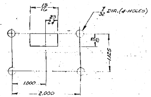
DETAIL N° 2 FULL SIZE
