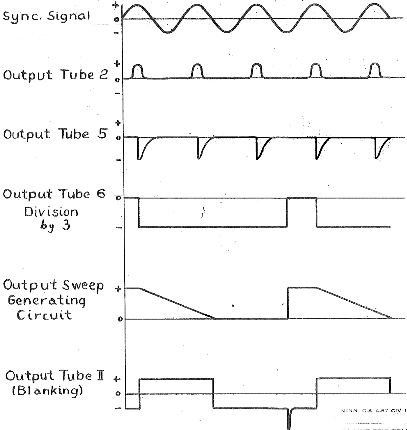
Wave Forms In Sweep Circuit
