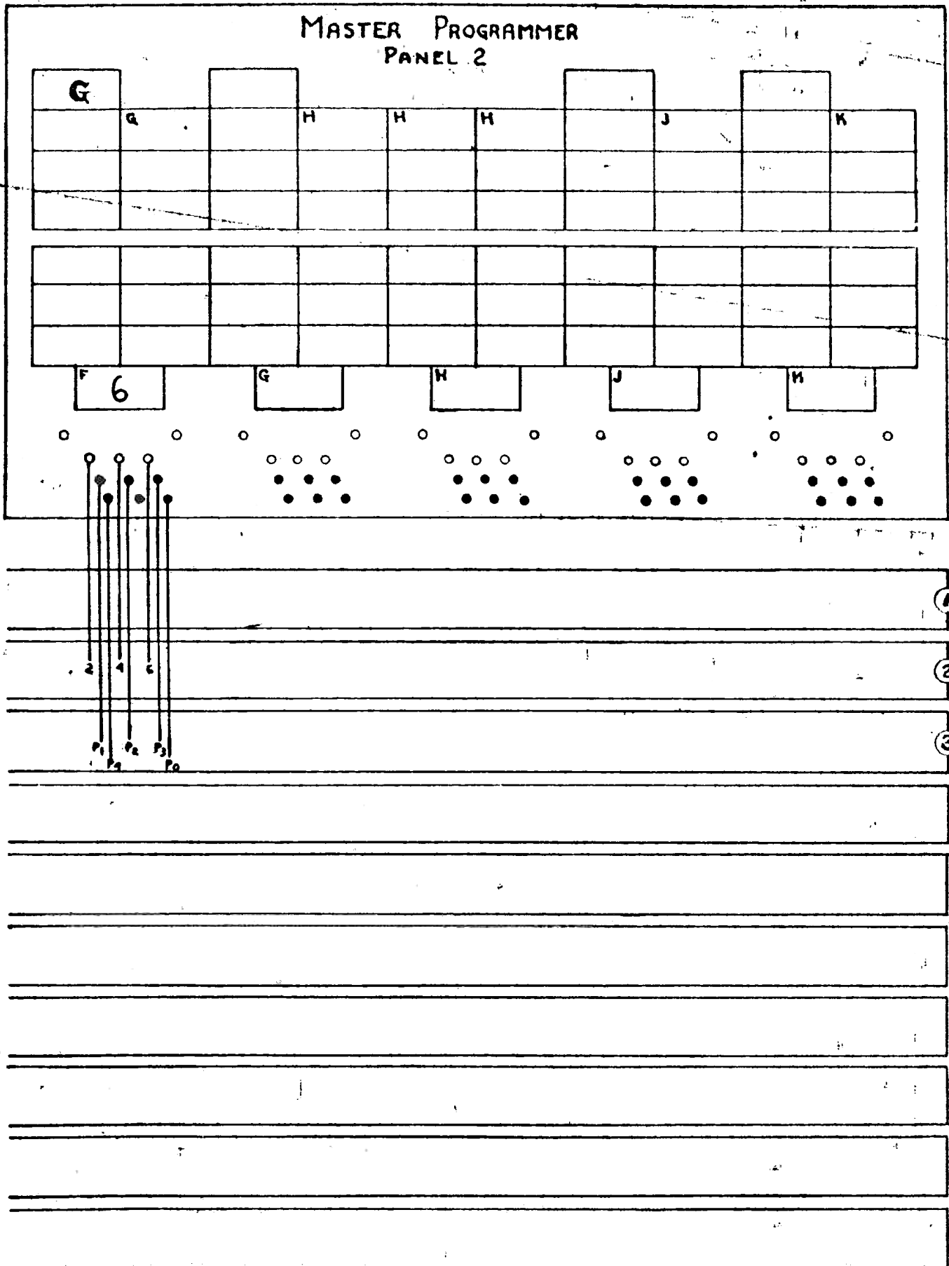
Fig. 10-2 (b) Digit Discrimination Program To stimulate P 1 if digit 1 appears in decade k of acc. 12
