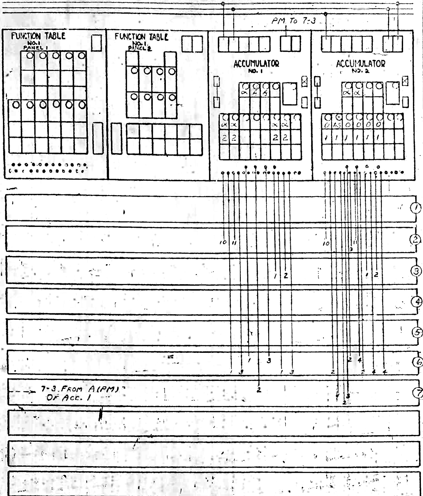
Fig. 10-9 (b). Set-Up Diagram For Tests on y and y^2 - Problem 2
