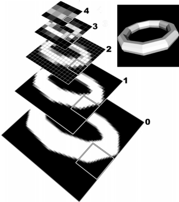
Figure 3: The hierarchy of occlusion maps. This particular hierarchy is created by recursively averaging over 2 blocks of pixels. The outlined square marks the correspondence of one top-level pixel to pixels in the other levels. The image also shows the rendering of the torus to which the hierarchy corresponds.
