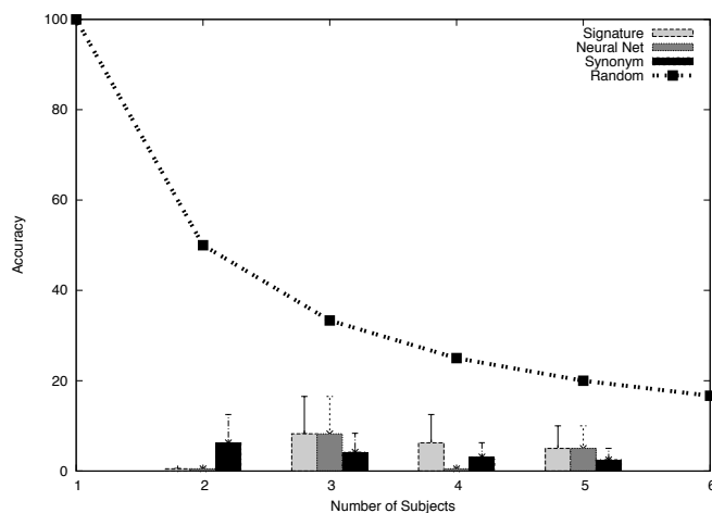
Fig. 3. Accuracy in detecting imitation attacks. The x-axis shows the number of subjects, the y-axis shows the average percentage of imitation attacks correctly classified. The error bars show the standard error for each experiment.
