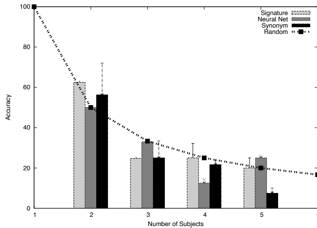
Fig. 2. Accuracy in detecting obfuscation attacks. The x-axis shows the number of subjects, the y-axis shows the average percentage of obfuscation attacks correctly classified. The error bars show the standard error for each experiment.
