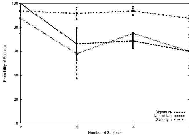
Fig. 4. Success rate of imitation attacks. The x-axis shows the number of subjects, the y-axis shows the average percentage of imitation attacks that were classified as being authored by the intended victim of the attack. The error bars show the standard error for each experiment.
