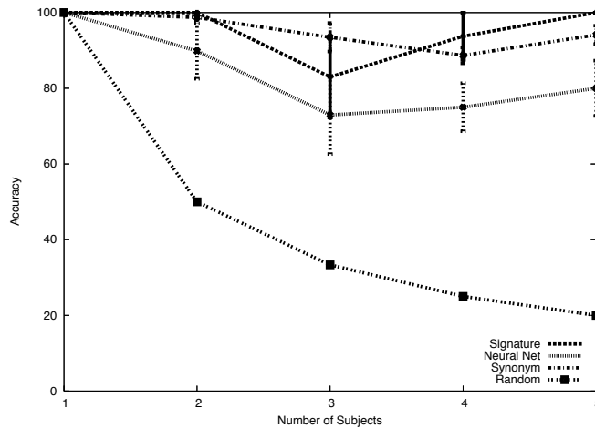
Fig. 1. Accuracy of the three methods without active attack. X-axis shows the number of subjects, y-axis shows the average percentage of documents correctly classified. Error bars show the standard error for each experiment.
